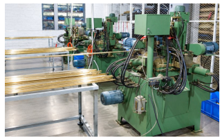
04 Stamping
